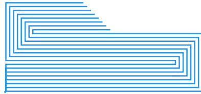
Fig. 2. Example paths of eight robots in benchmark coverage sweep. Robots begin in the bottom left, then sweep until locating where v \leq v^* and all robots know the location.
