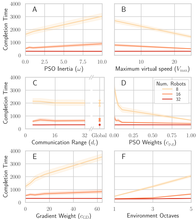
Fig. 3. Parameter effects on time (in ticks) for first robot to locate target, for 5 octave environment. Lines and shading show median and 25th/75th percentiles, respectively.
